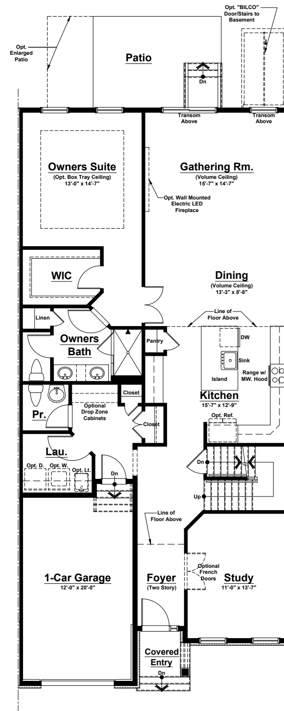
FLOORPLAN SHOWN IS ELEVATION #1
