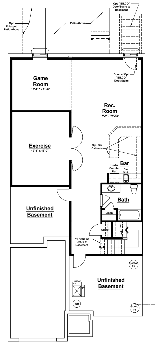
OPTIONAL FINISHED BASEMENT
