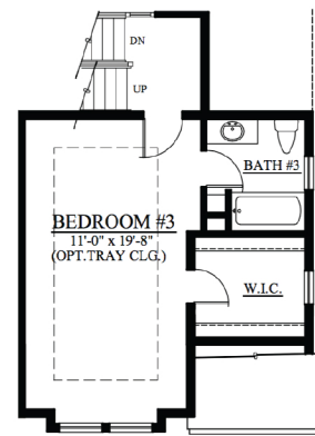
MID. FLOOR ELEVATION #1
